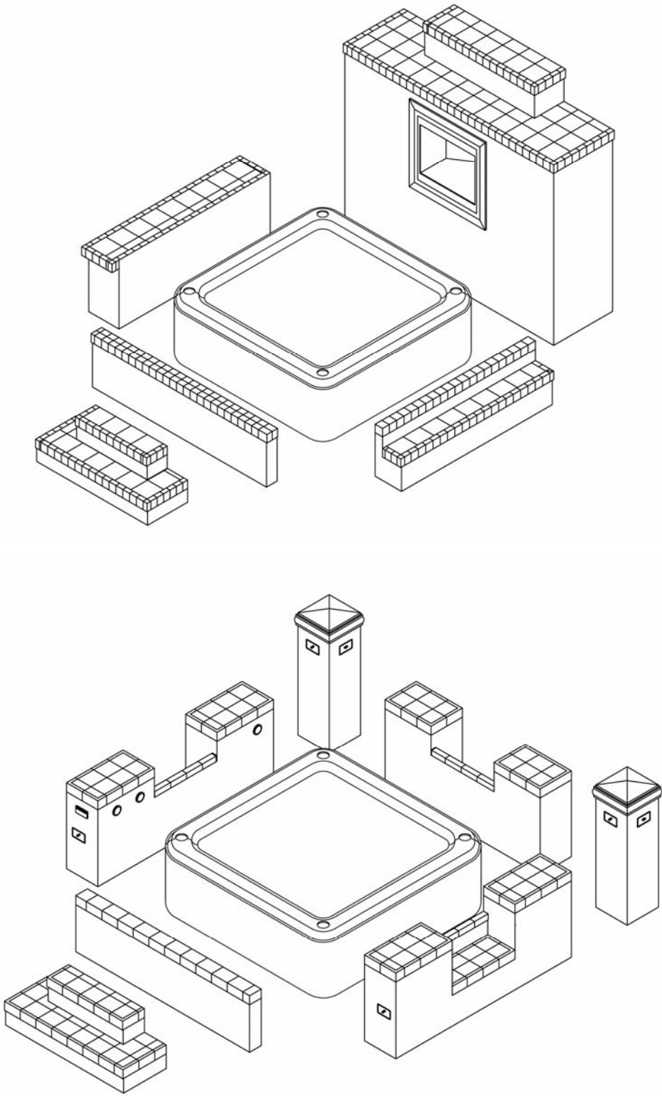
Figure 1. Exploded view of SW-100 and SW-400
