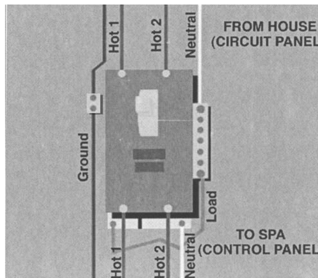
Figure 2. GFCI Hook-Up
